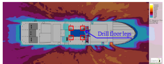
Fig. 5 Fire analysis results : 150 kg/s release on the drill floor is ignited and 5.4 m/s wind blows from aft (scenario no. 4)
