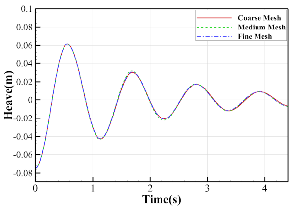
(b) Heave decay curves for cylinder
