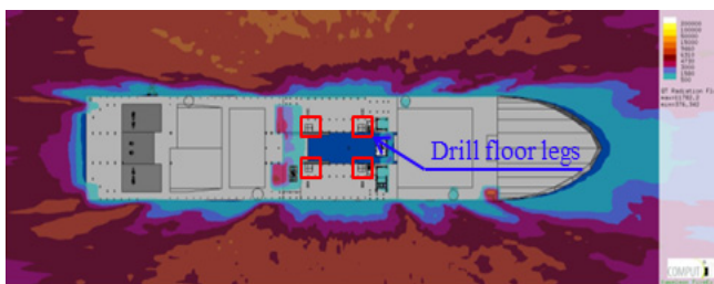
Fig. 3 Fire analysis results : 150 kg/s release on the drill floor is ignited and 5.4 m/s wind blows from forward (scenario no. 2)
