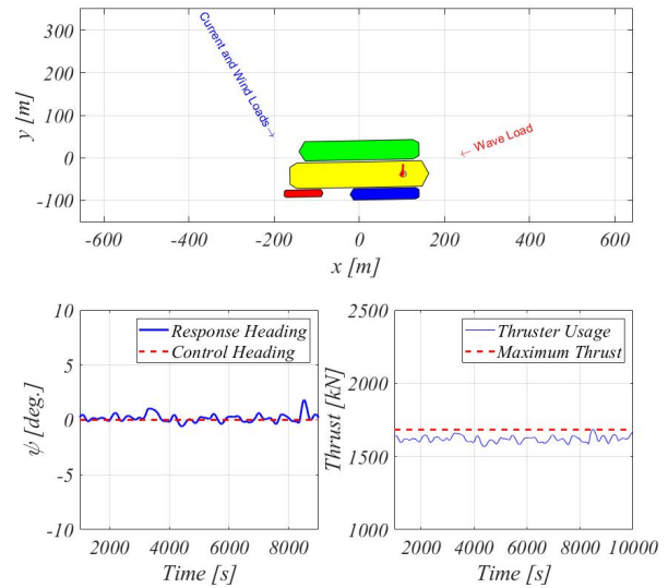
(b) Simulation case (Current and wind loads direction 300°)
