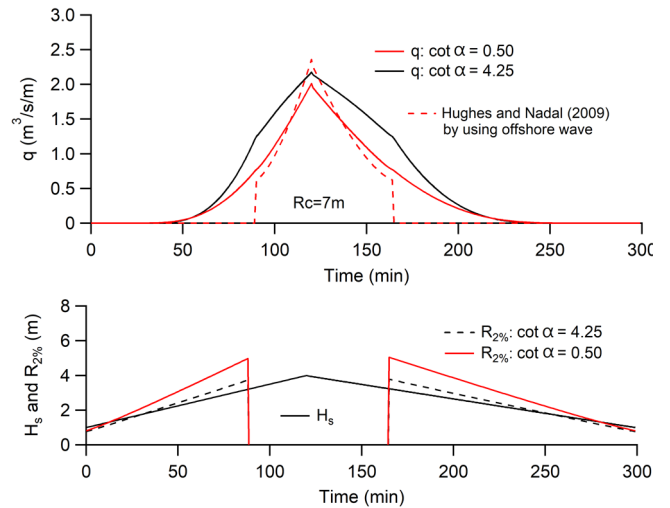
Fig. 6 Wave runup height and inundation flow toward coastal seawall located on shoreline
