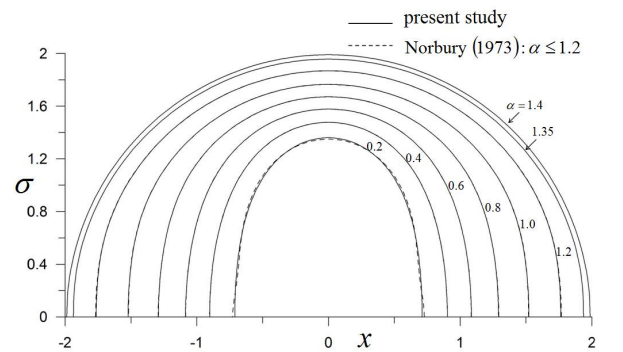
Fig. 7 Shapes of dividing stream surface for various values of \alpha
